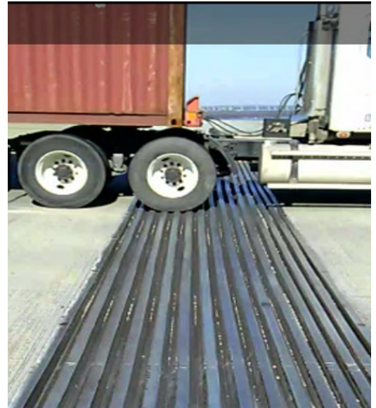
Figure 2: The Arthur Ravenel Bridge, Charleston SC, incorporates 54" SSB joints
